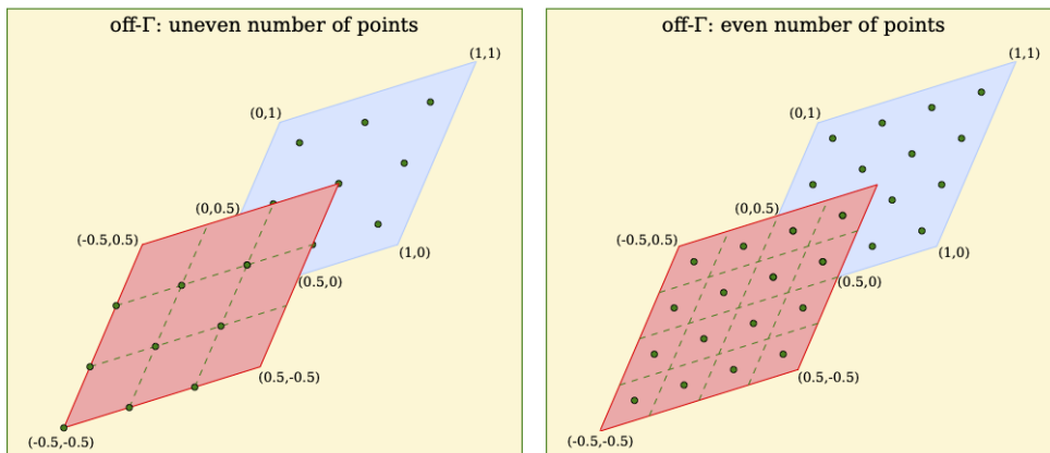
Figure 4.3: The Monkhorst Pack grid [216] in two dimensions for even and uneven numbers of grid points. In the left picture (uneven number of grid points) the \Gamma point is included in the grid.
